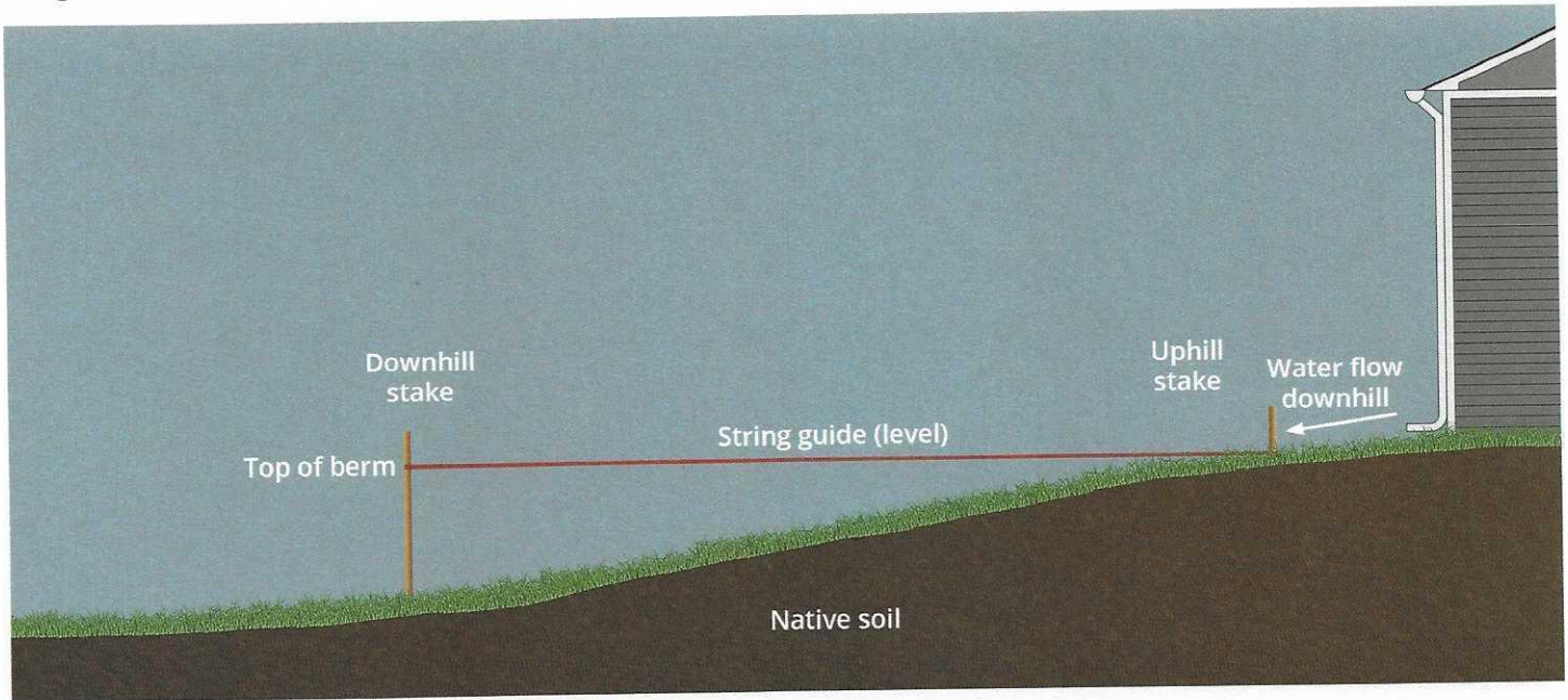
Figure 3. The string should be tied to the base of the uphill stake, then tied to the downhill stake at the same level.
